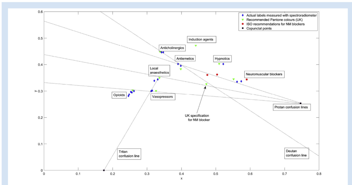
Fig 2. CIE 1931 colour space showing chromaticities of labels recorded by spectroradiometry (diamonds), colours recommended by the UK guidance (triangles), and colours recommended by ISO standard. Any pair of chromaticities lying on a line that passes through a copunctal point are potentially confusable. The deutan co-punctal point is out of the bounds of this plot at x=1.4 , y=-0.4 . Confusion lines are illustrated for chromaticity pairs described in the text. ISO, International Organization for Standardization.
