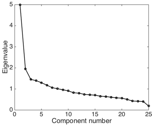
Fig. 1. Scree plot.
